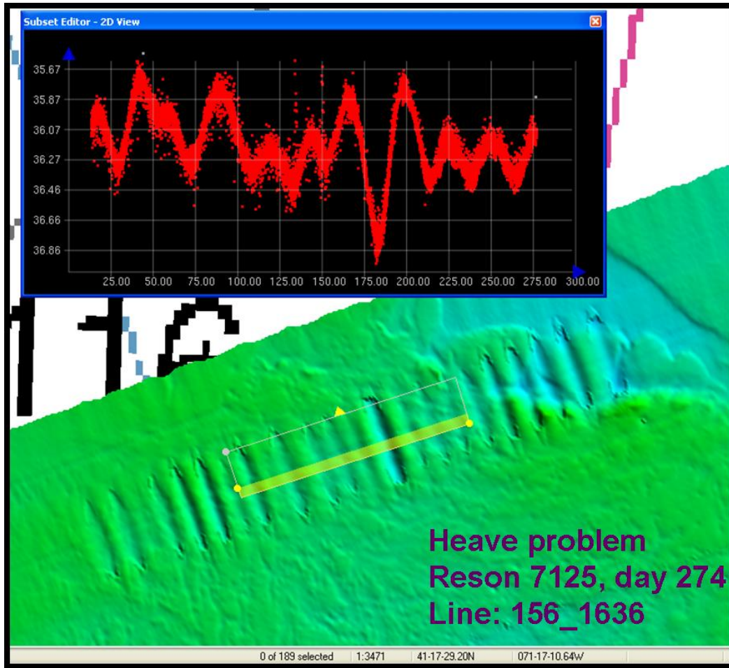
Figure B-2: heave artifact line 156_1636.
